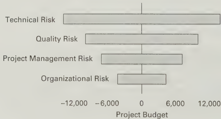
FIGURE 6.5 Tornado diagram
