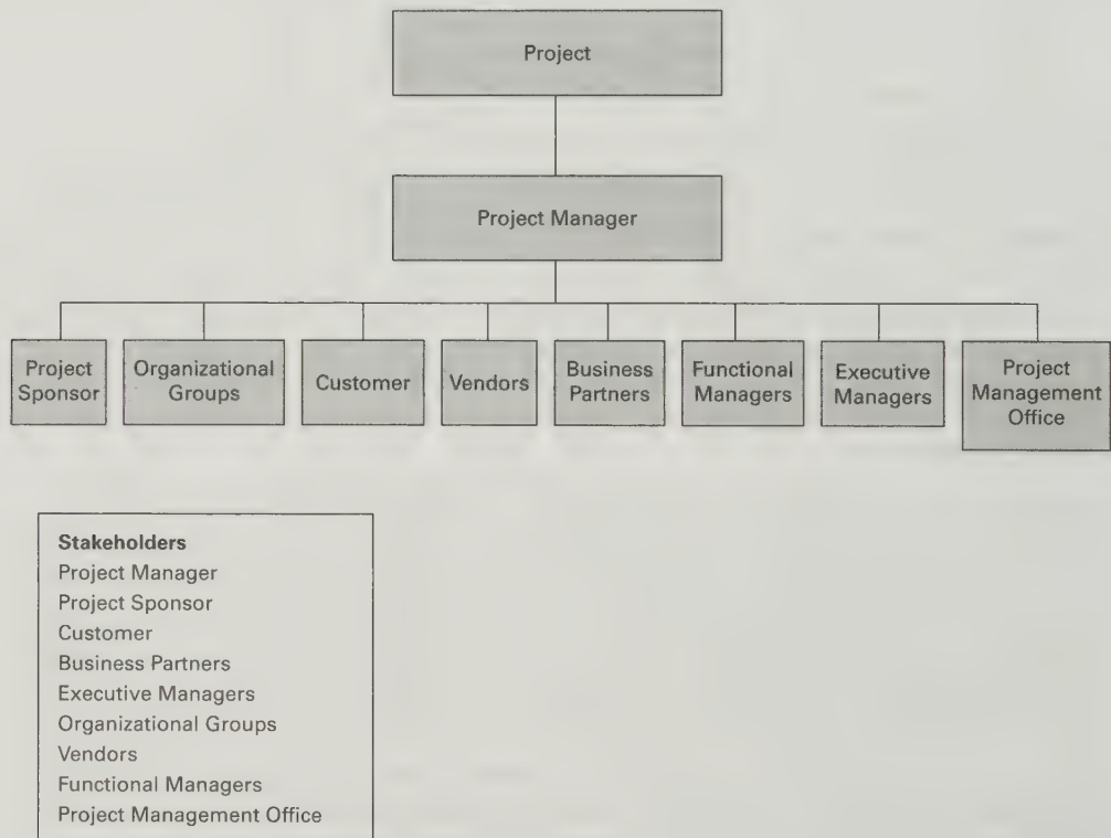
FIGURE 1.1 Project stakeholders
