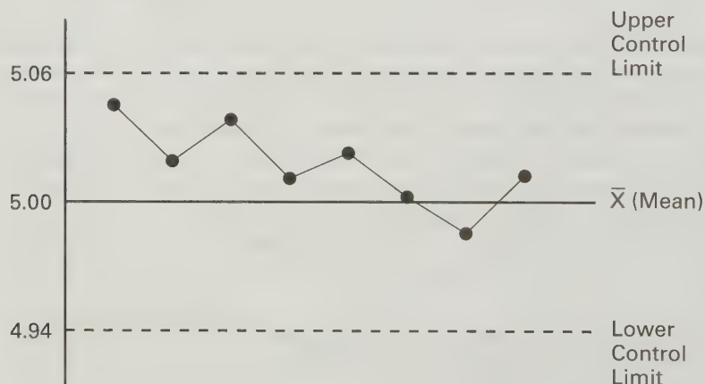
FIGURE 11.2 Control chart
