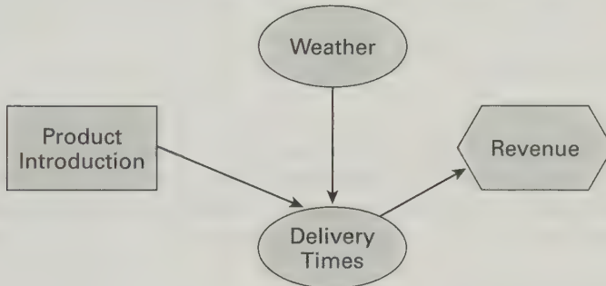
FIGURE 6.4 Influence diagram
