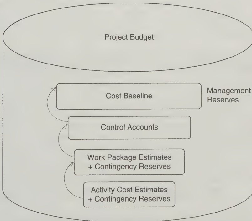
FIGURE 5.1 Project budget
