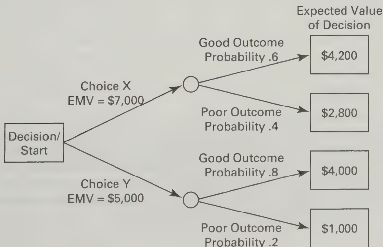
FIGURE 6.6 Decision tree
