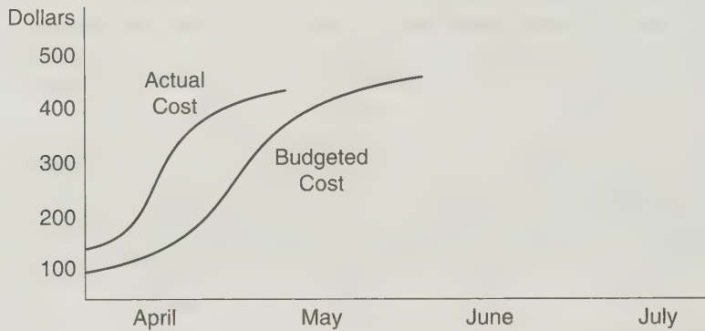
FIGURE 5.2 Cost baseline
