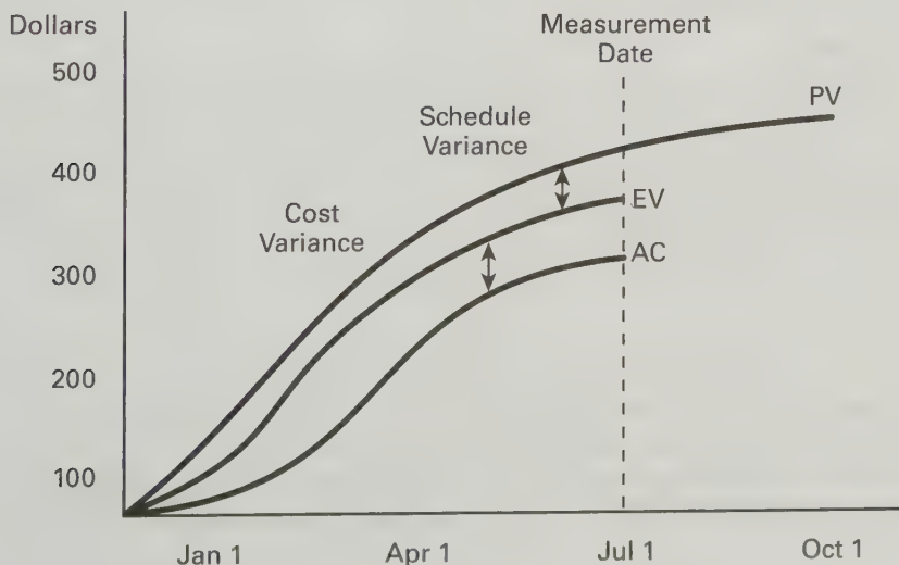
FIGURE 11.1 Earned value
