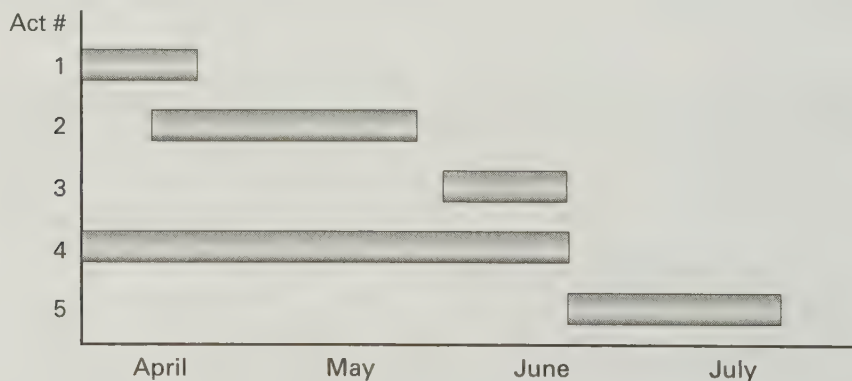
FIGURE 4.5 Gantt chart
